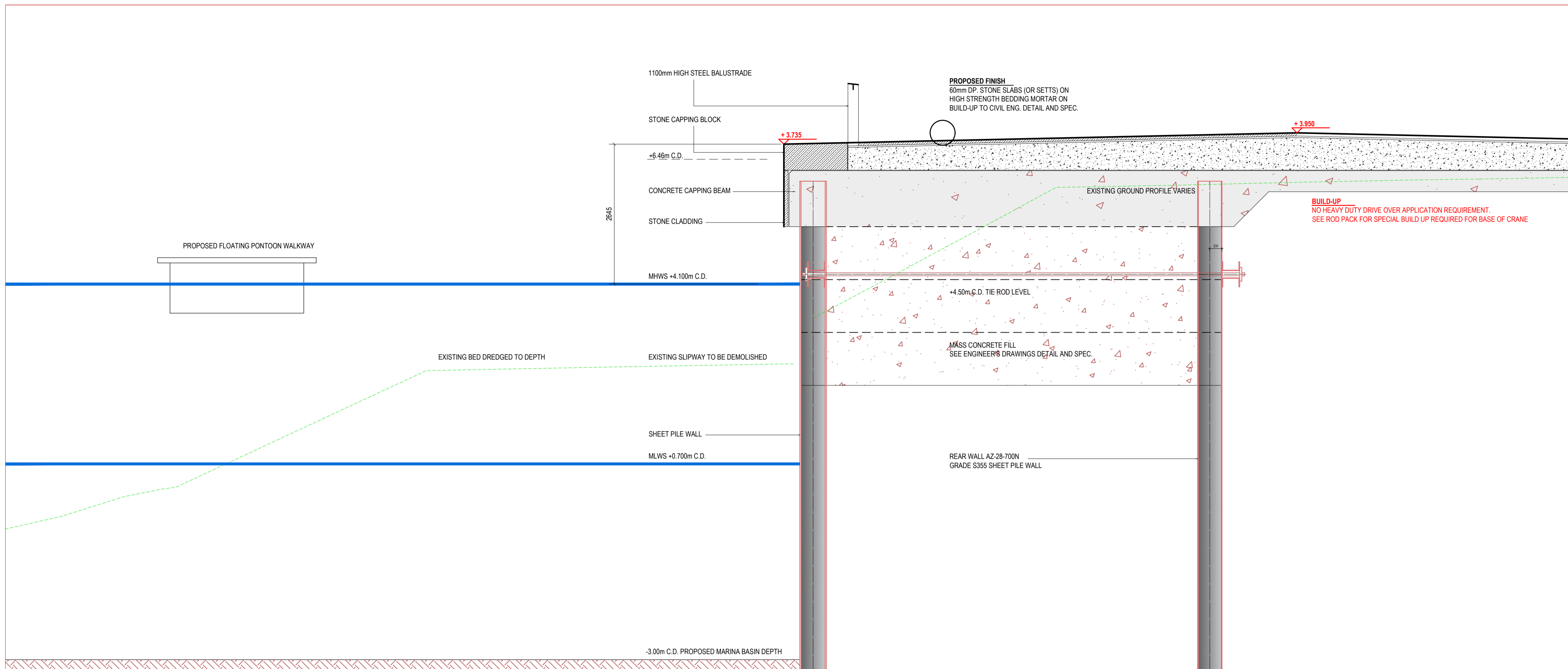
01. SECTION 01, WEST QUAY WALL
