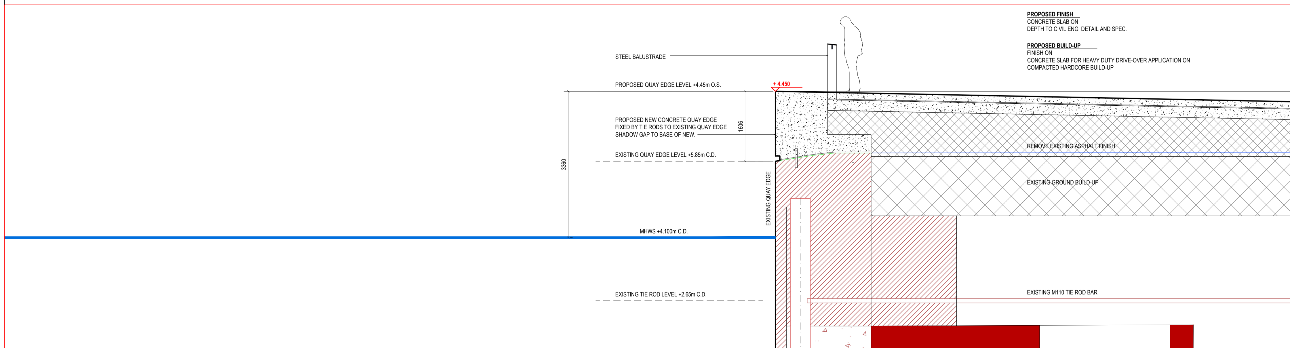
02. SECTION 04, QUAY WALL, (EXISTING)
