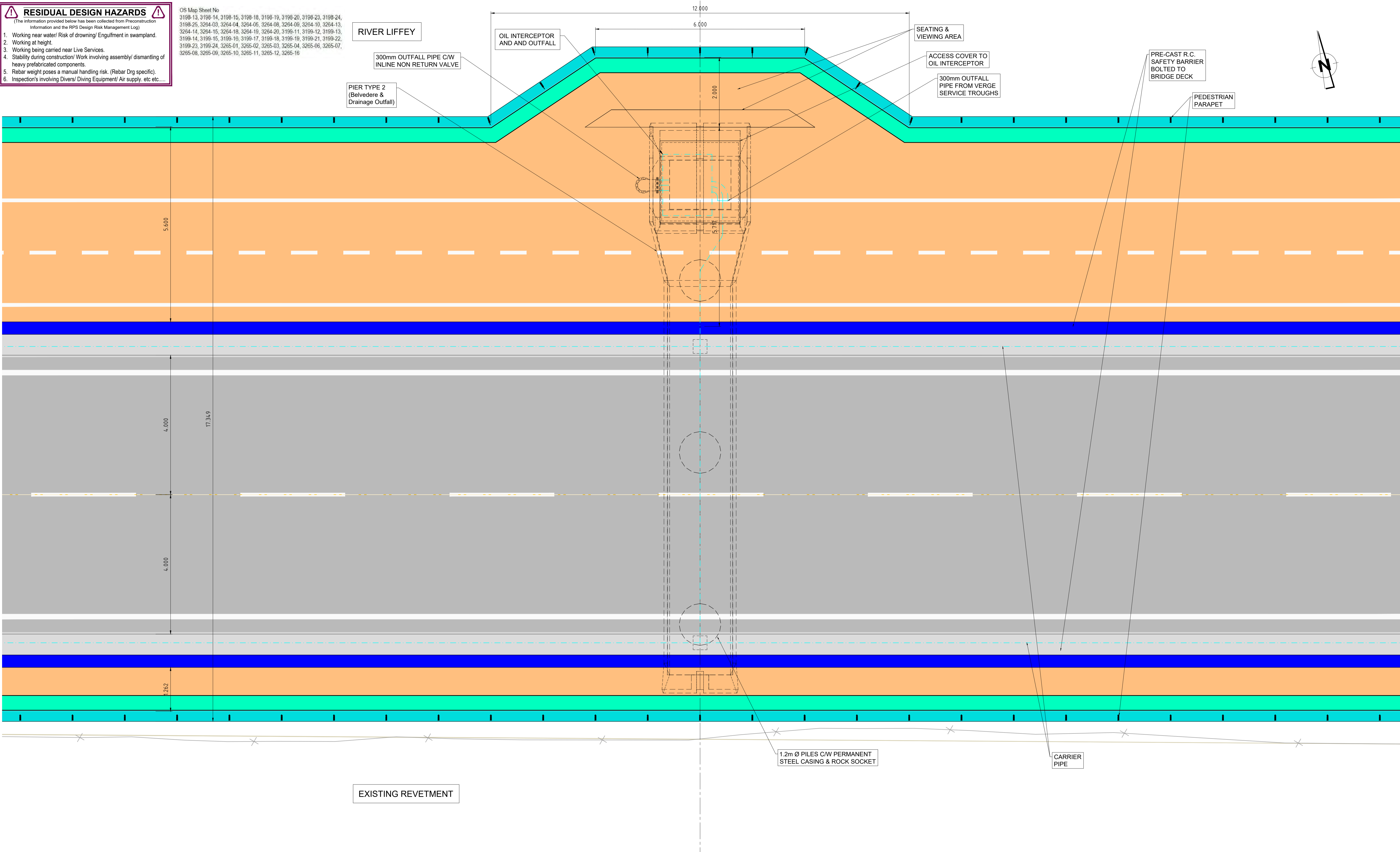
PLAN LAYOUT - BELVEDERE & DRAINAGE OUTFALL (Scale 1 : 50)
