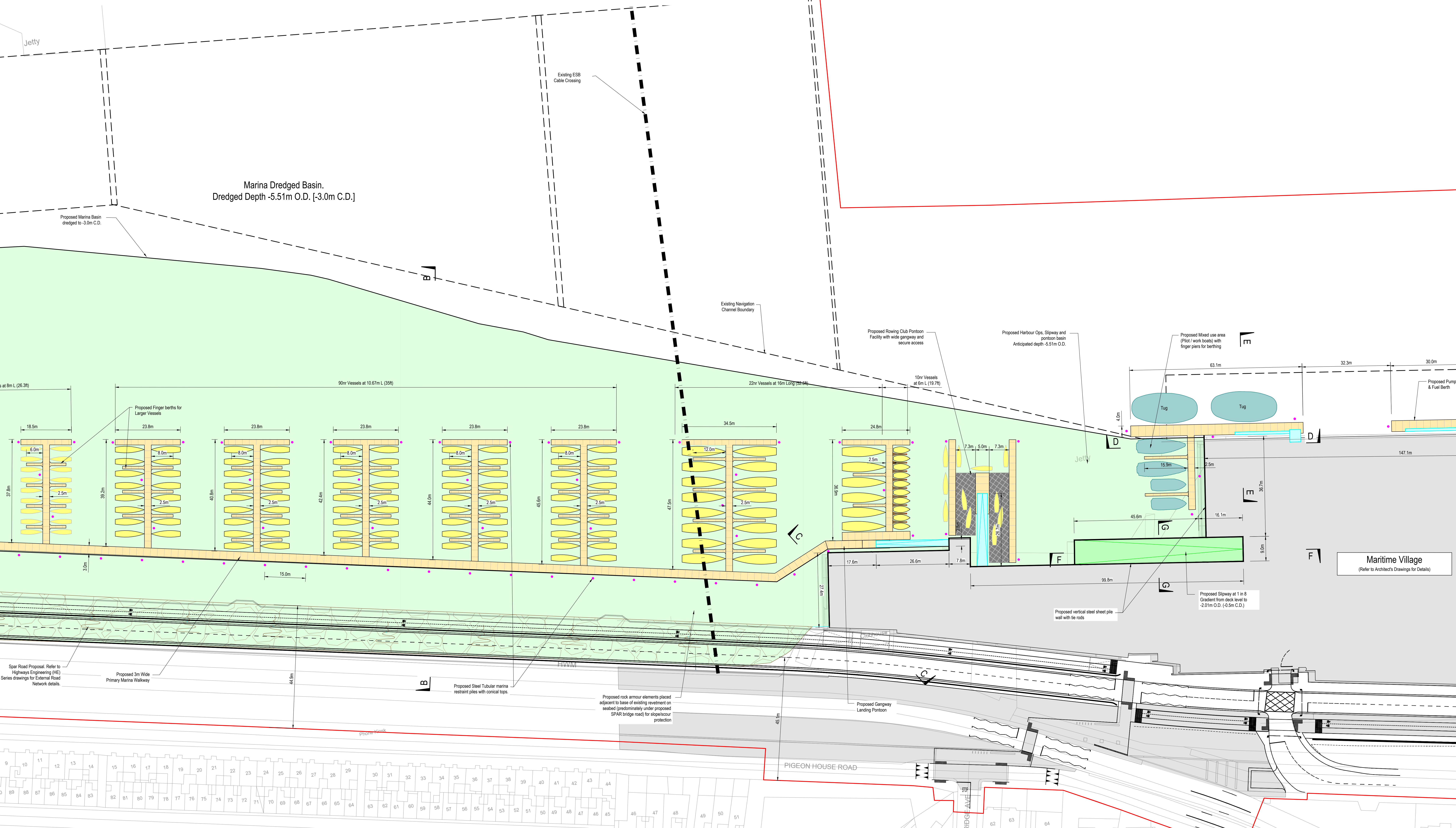
Maritime Village Proposed Marina Layout - Sheet 2 [1:500]
