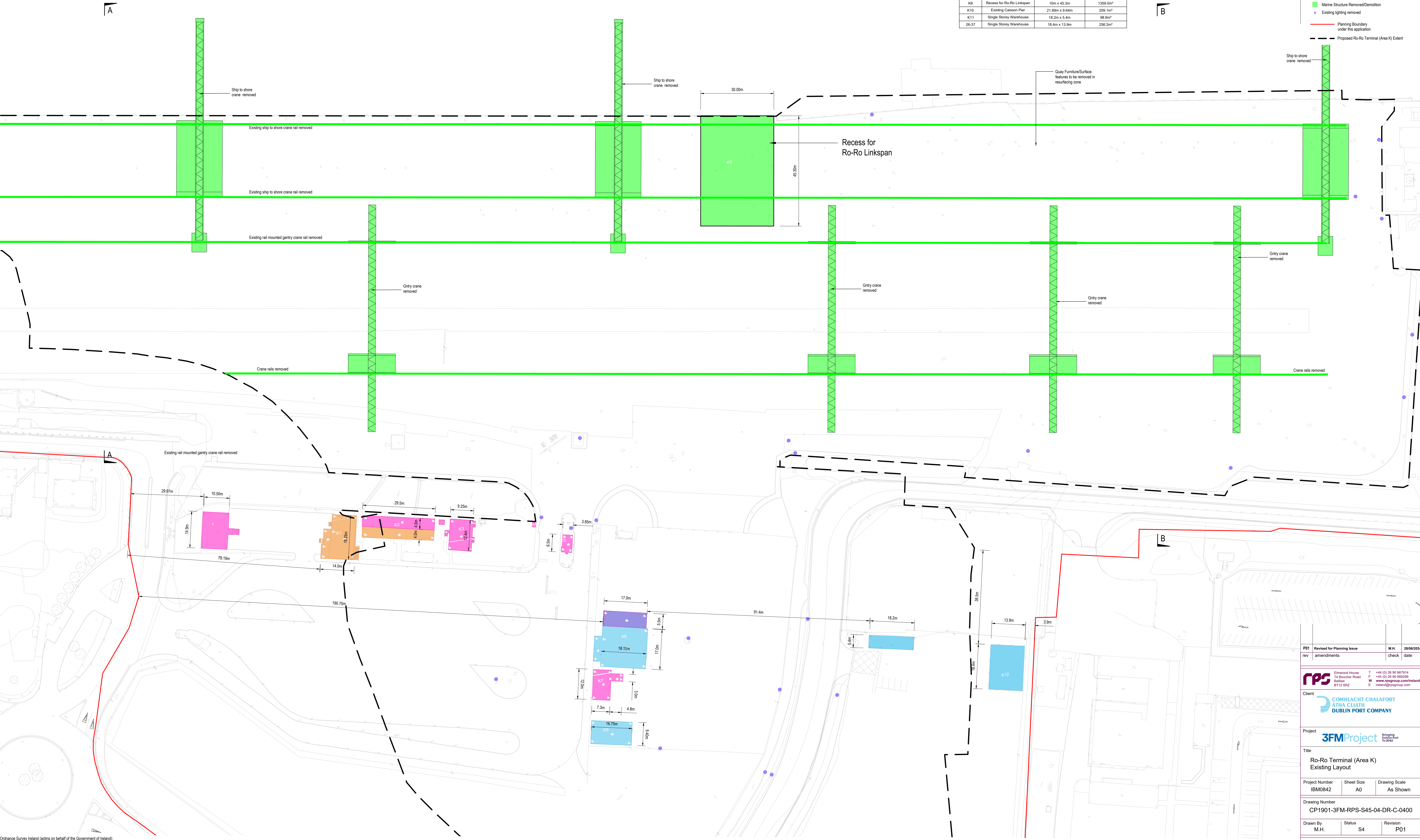
Existing Layout with Building and Marine Structure Demolition Plan [1:500]
