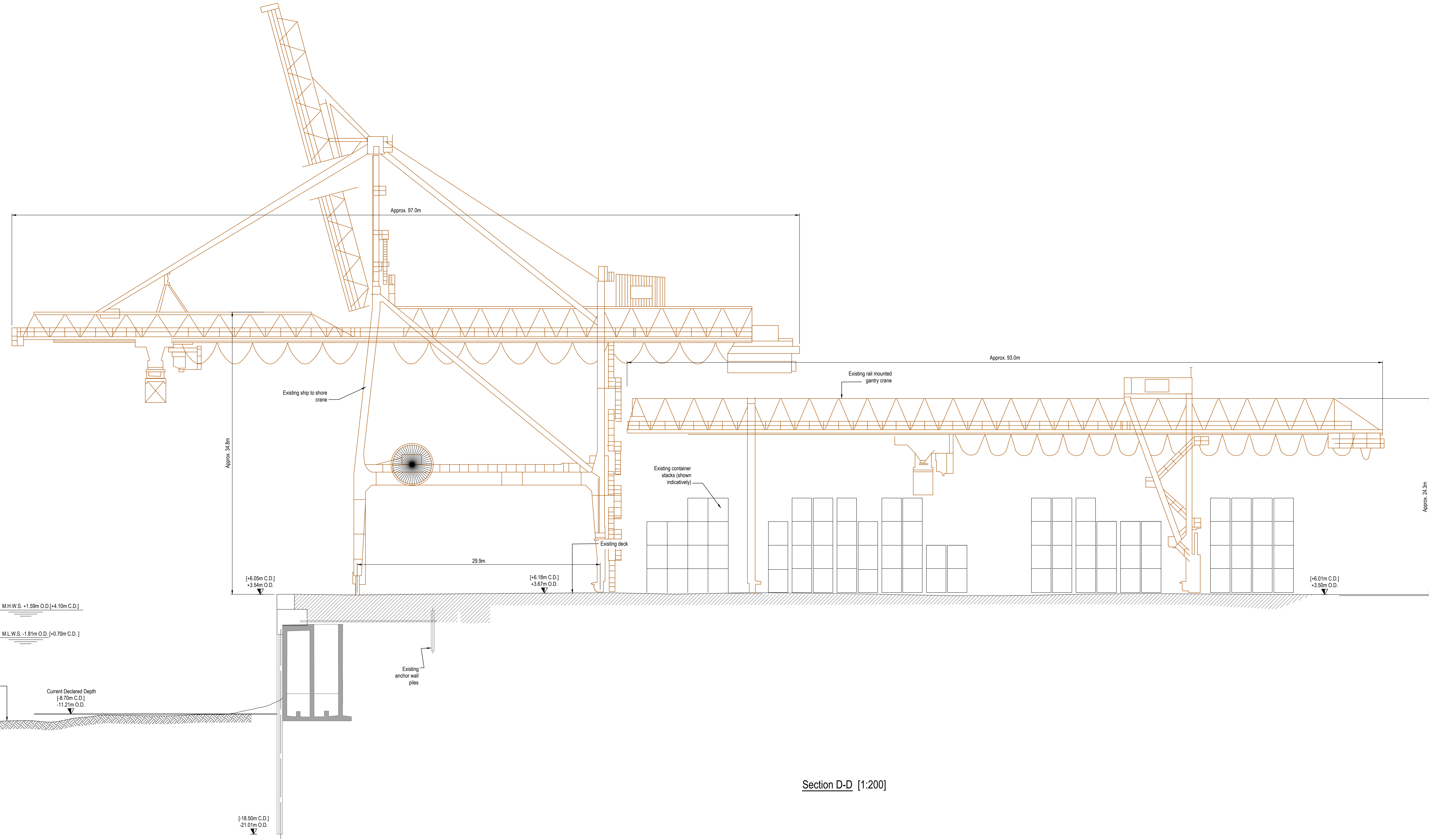
Key Plan Showing Section Locations [1:2500]
