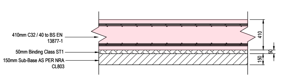
Area 1 - Container Stack Pavement Detail [1:25]
