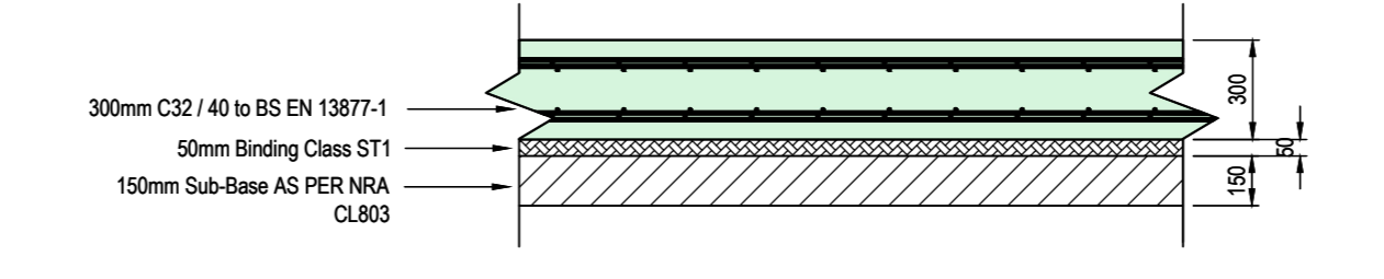
Area 2 - HGV/Tractor and Trailer Heavy Duty Pavement Detail - Option 1 Concrete [1:25]
