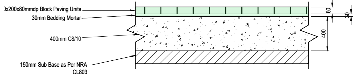
Area 2 - HGV/Tractor and Trailer Heavy Duty Pavement Detail - Option 2 Pavers [1:25]
