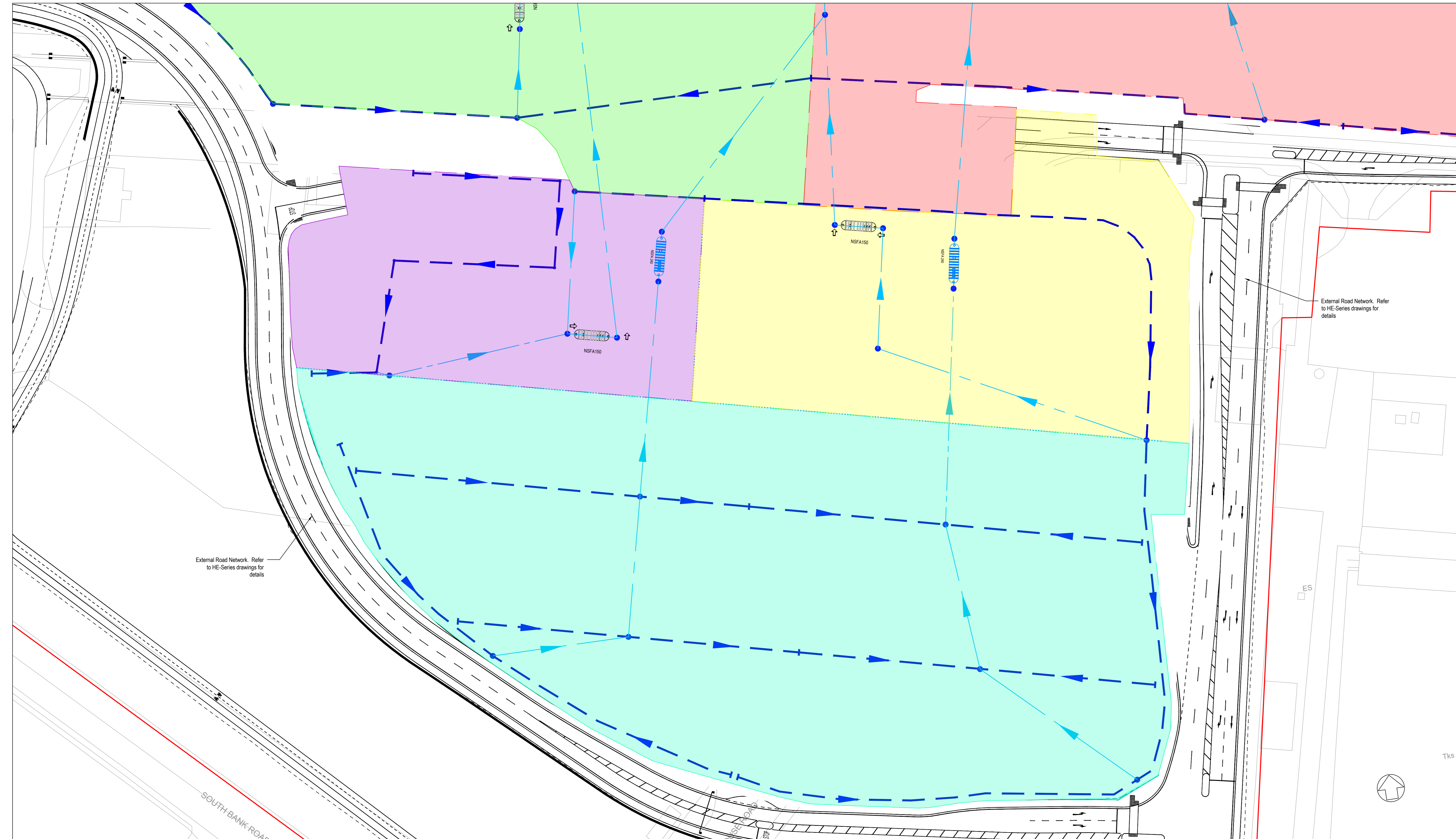
Proposed Drainage Layout [1:500]
