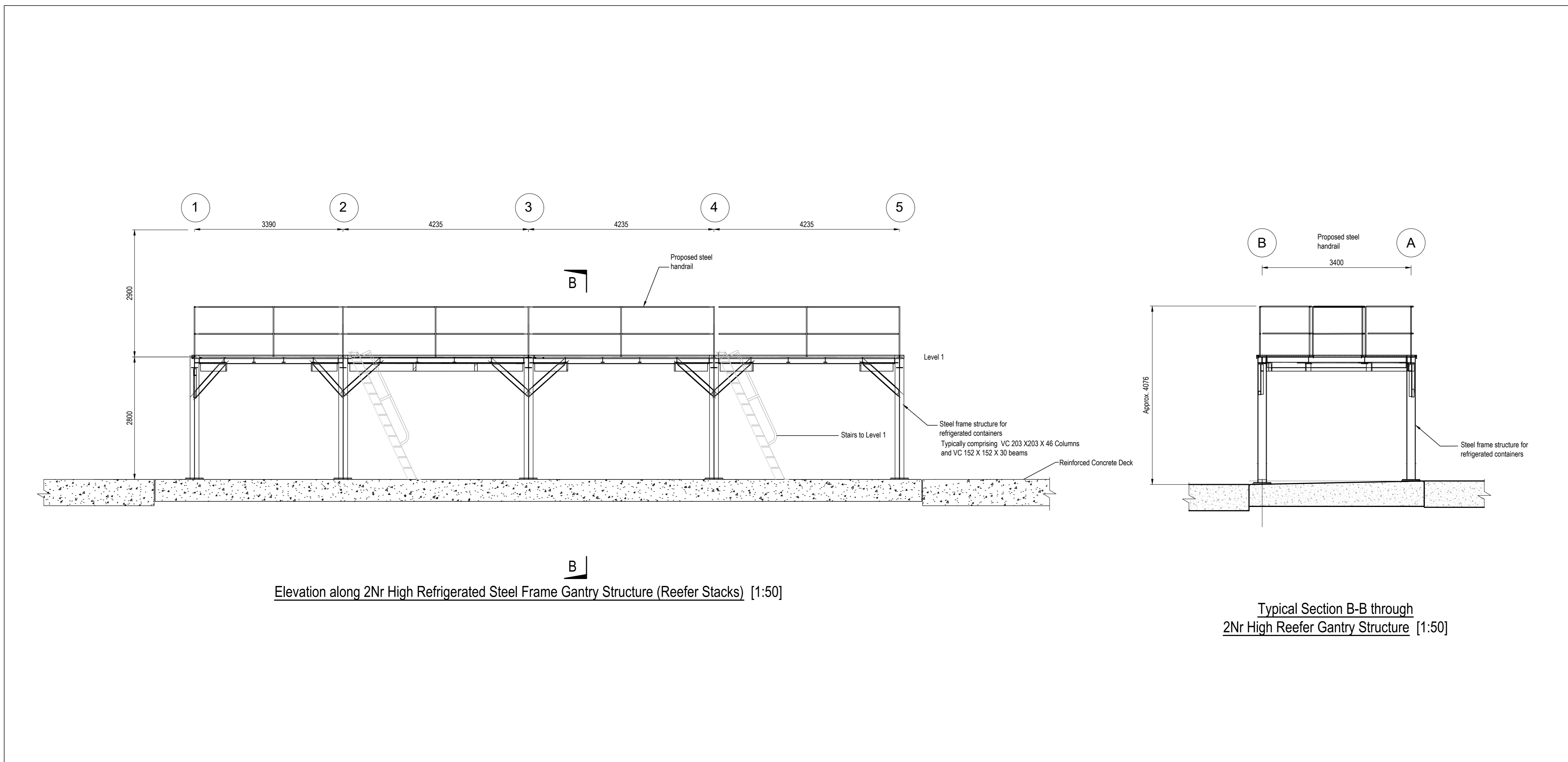
Typical Section A-A through 6Nr High Reefer Gantry Structure [1:50]
