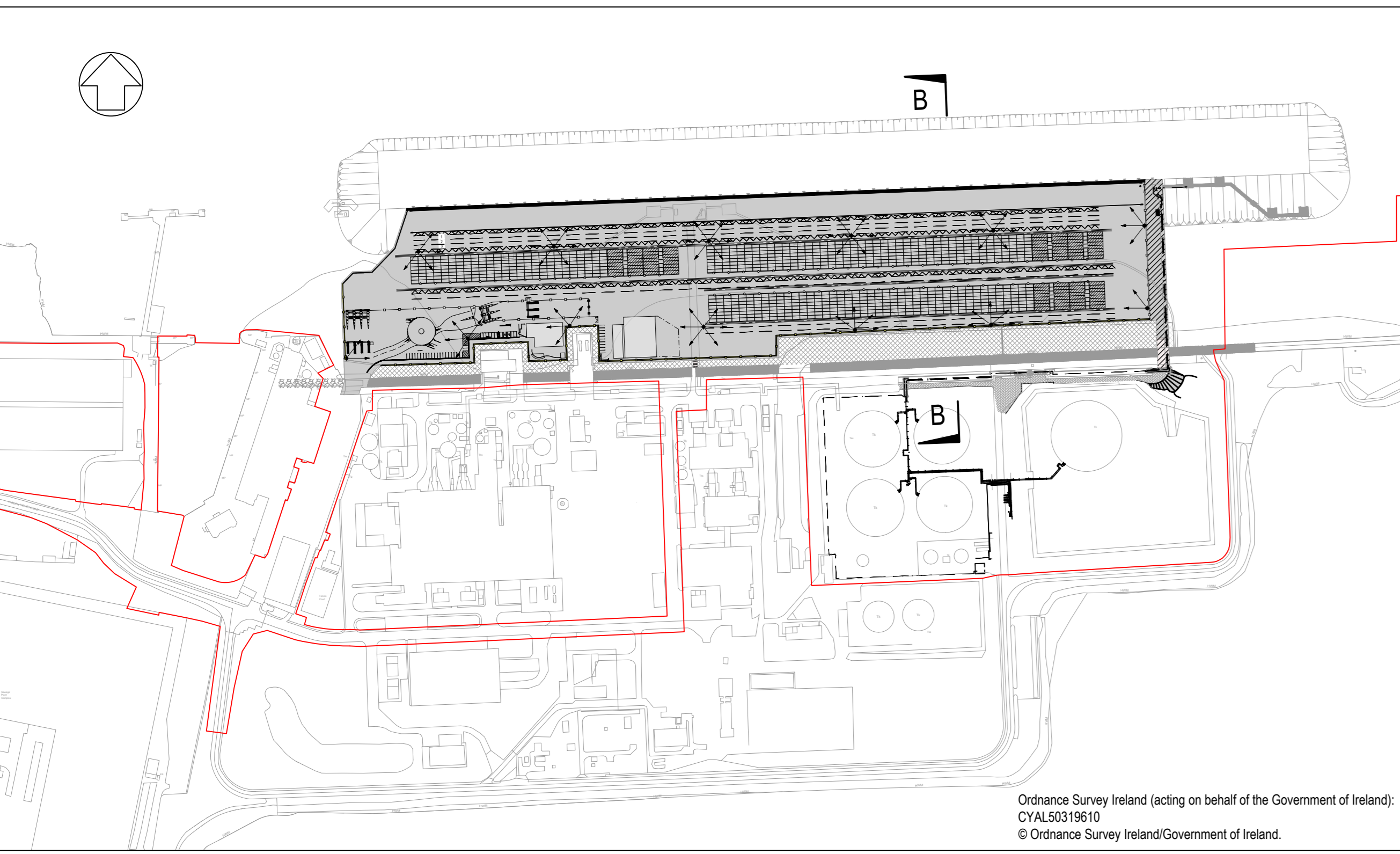
Key Plan showing Section Location [1:2500]
