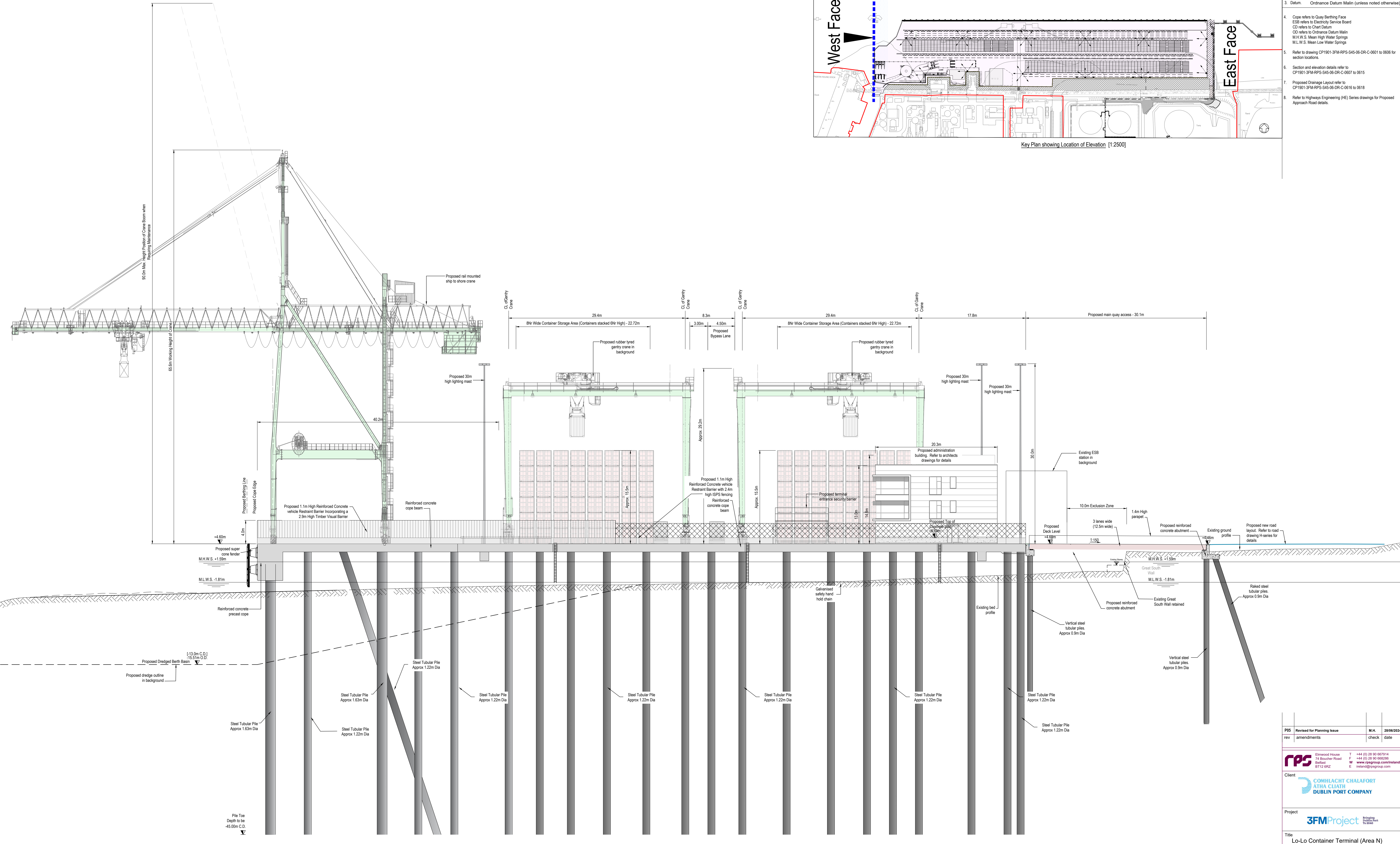
West Elevation [1:200]
