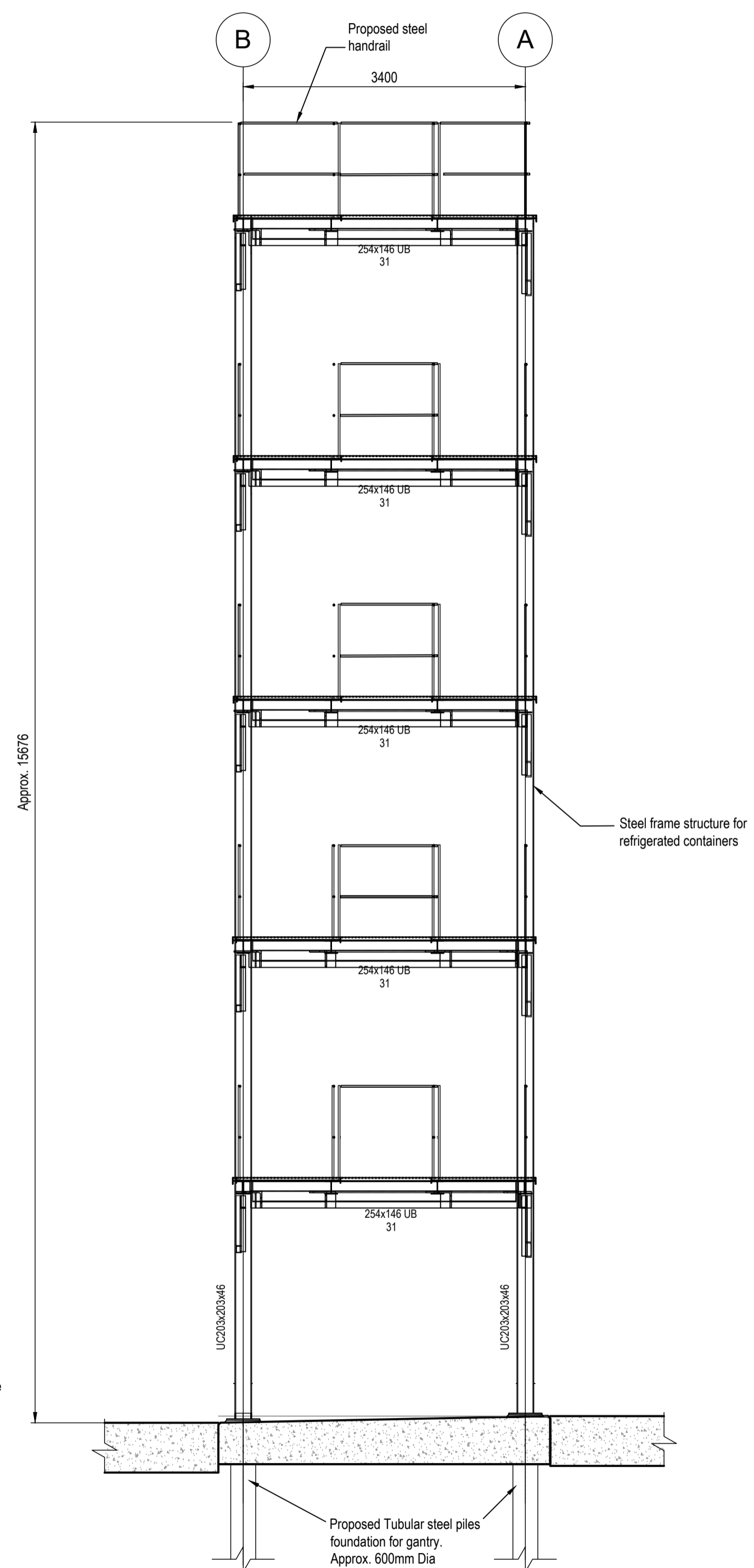
Typical Section A-A through Reefer Gantry Structure [1:50]
