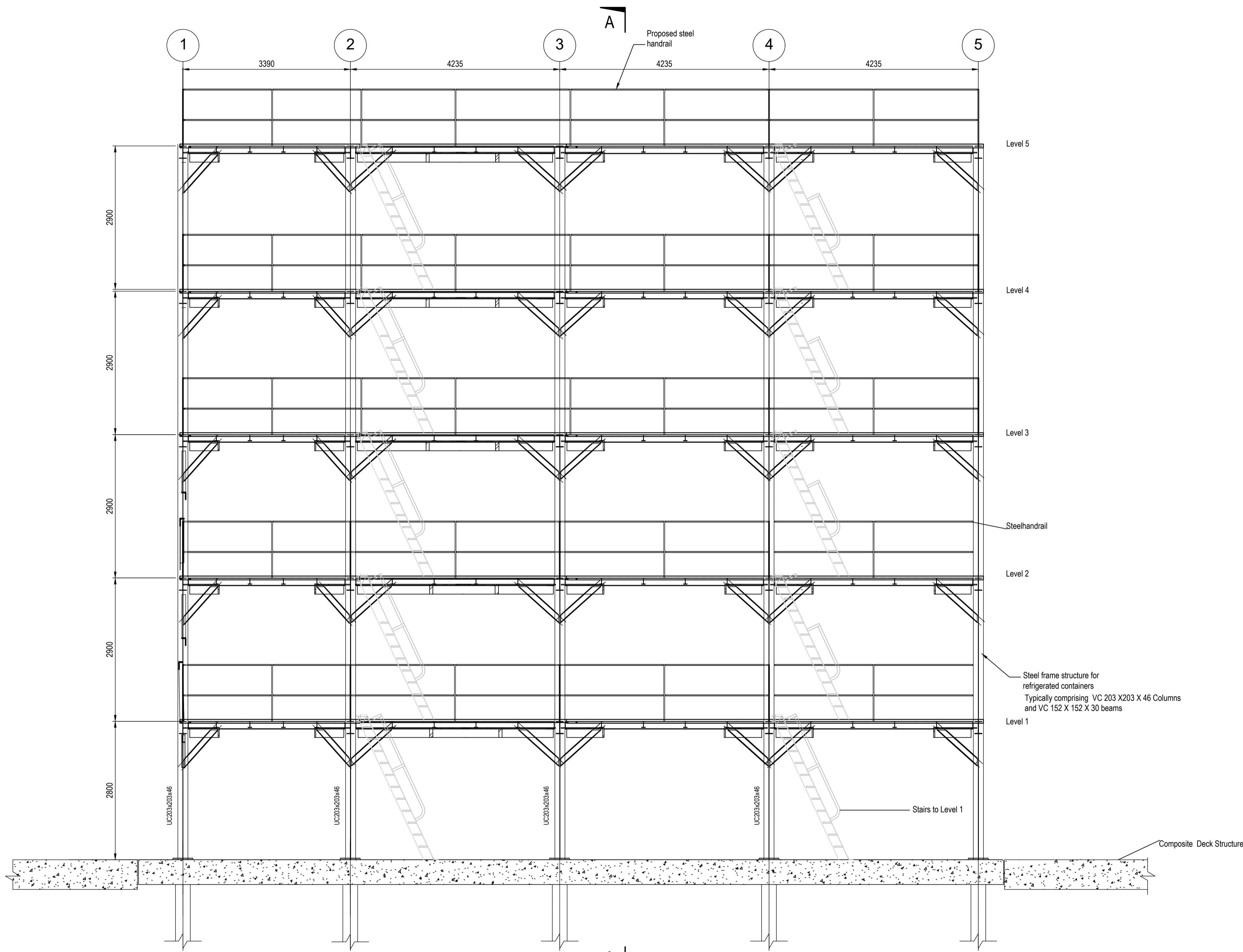
Elevation along Refrigerated Steel Frame Gantry Structure (Reefer Stacks) [1:50]
