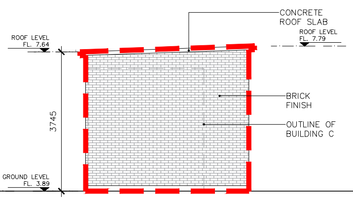
6 Existing Substation Building - North Elevation EX-B-100 1:100
