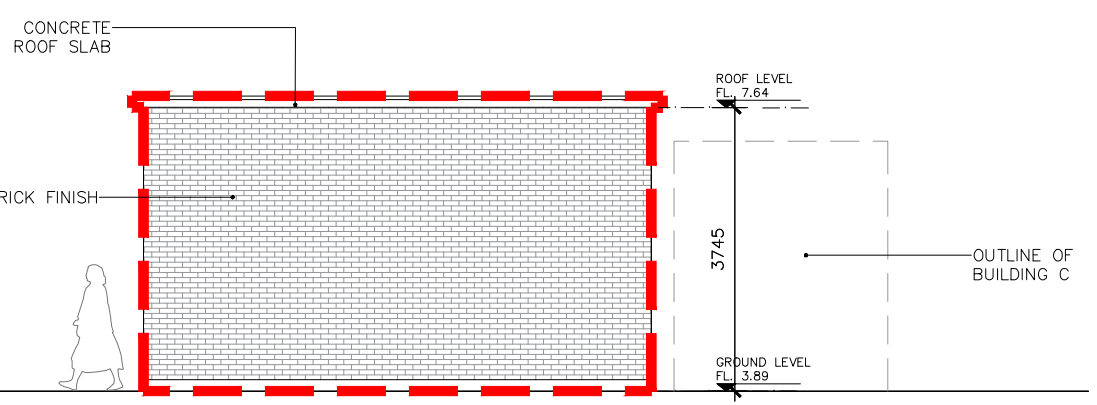
5 Existing Substation Building - East Elevation EX-B-100 1:100
