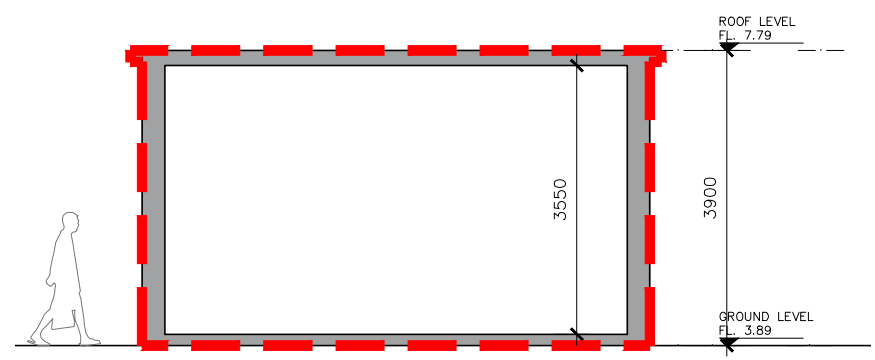
7 Existing Substation Building - Section A-A EX-B-100 1:100
