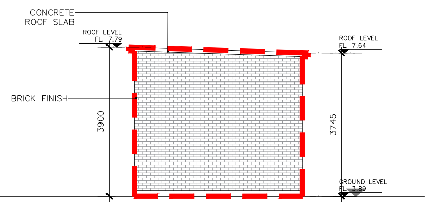
4 Existing Substation Building - South Elevation EX-B-100 1:100
