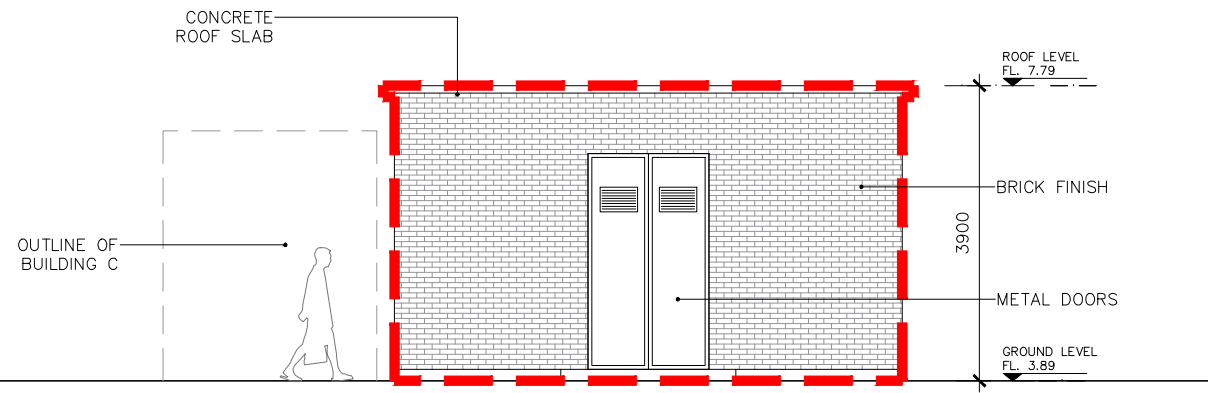
3 Existing Substation Building - West Elevation EX-B-100 1:100
