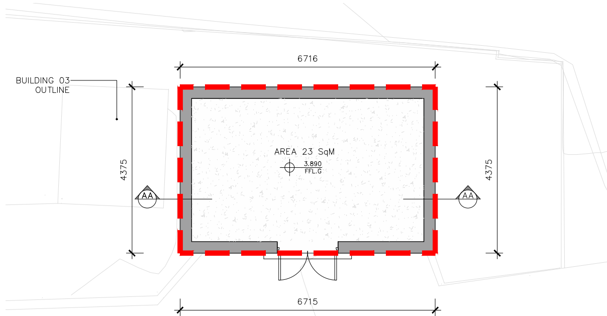
1 Existing Substation Building - Ground Floor Plan EX-B-100 1:100
