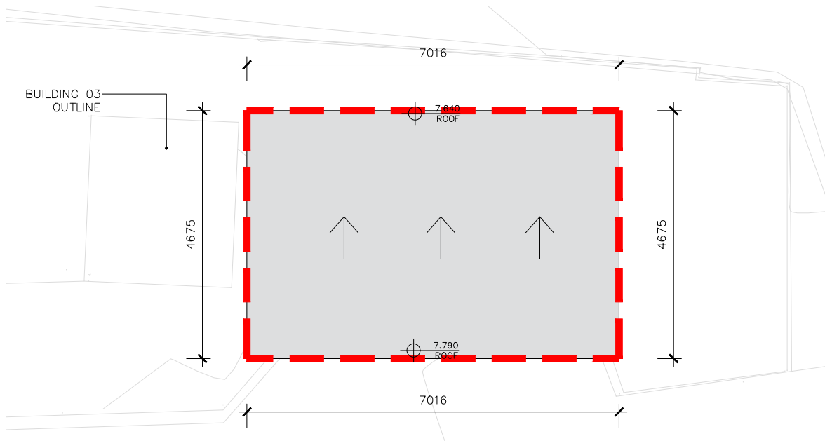
2 Existing Substation Building - Roof Plan EX-B-100 1:100
