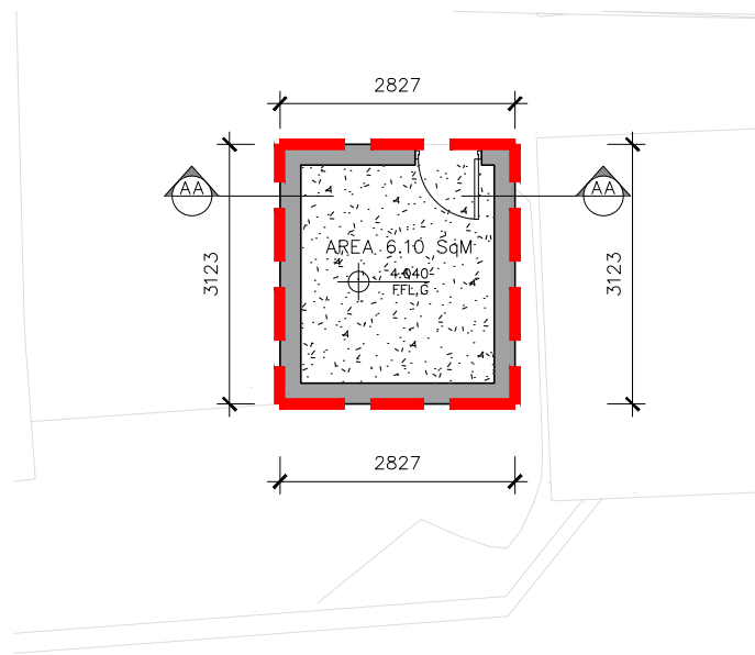
1 Existing Substation Building C - Ground Floor Plan EX-C-100 1:100
