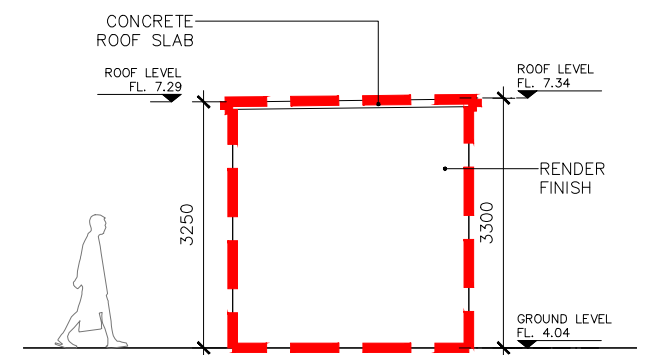
7 Existing Substation Building C - South Elevation EX-C-100 1:100
