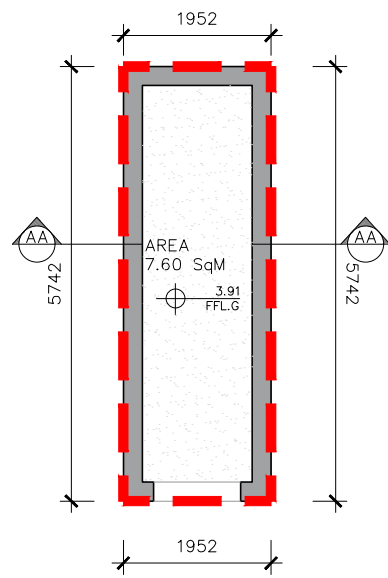
1 Existing Ancillary Building E - Ground Floor Plan EX-E-100 1:100
