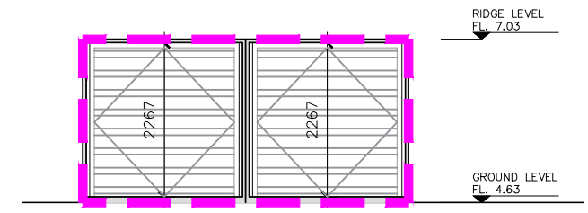
6 Existing Container Structure F2 - Section A-A EX-F-100 1:100
