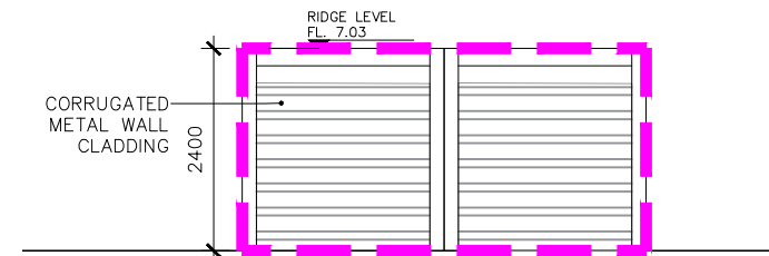
9 Existing Container Structure F1 - East Elevation EX-F-100 1:100
