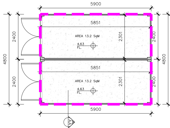
3 Existing Container Structure F2 - Ground Floor Plan EX-F-100 1:100
