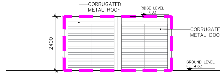
7 Existing Container Structure F1 - West Elevation EX-F-100 1:100
