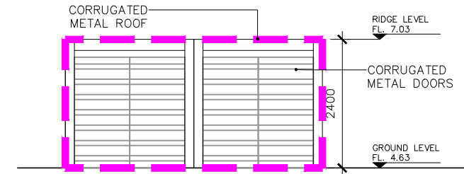
8 Existing Container Structure F2 - West Elevation EX-F-100 1:100
