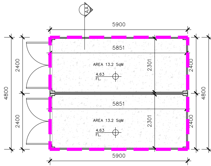
1 Existing Container Structure F1 - Ground Floor Plan EX-F-100 1:100
