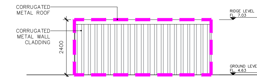
11 Existing Container Structure F1 - North Elevation EX-F-100 1:100
