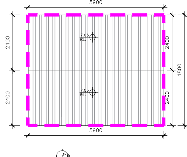
4 Existing Container Structure F2 - Roof Plan EX-F-100 1:100
