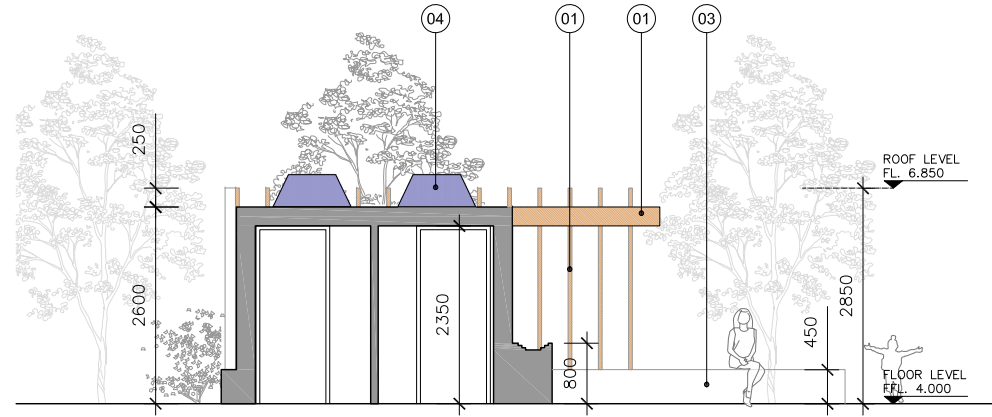
04 Proposed Section AA PA100 1:100
