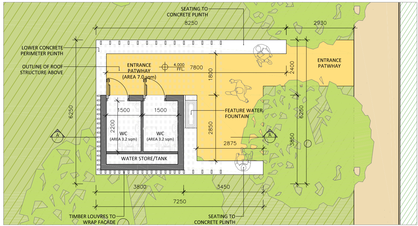
03 Proposed Floor Plan PA100 1:100
