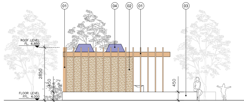
02 Proposed South Elevation PA100 1:100
