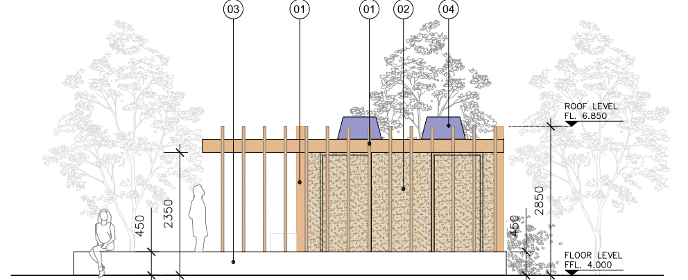
06 Proposed North Elevation PA100 1:100
