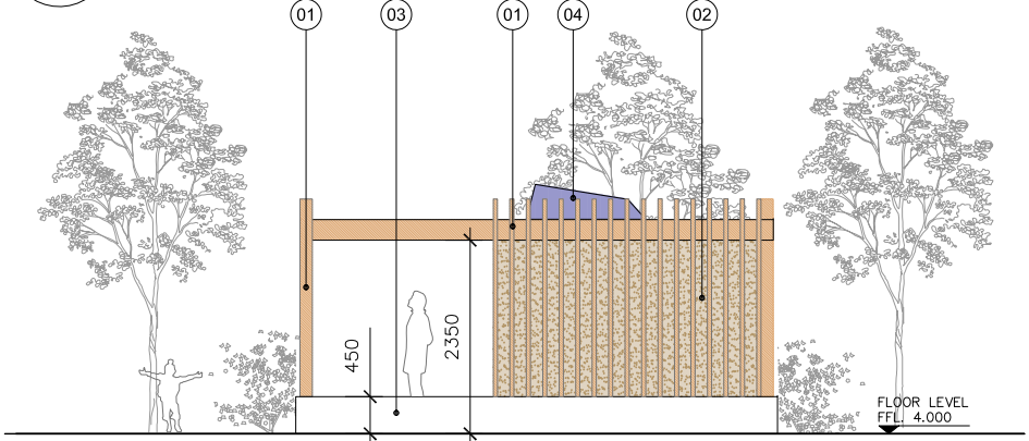
05 Proposed West Elevation PA100 1:100
