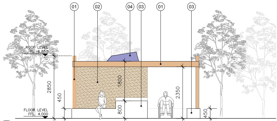
01 Proposed East Elevation PA100 1:100
