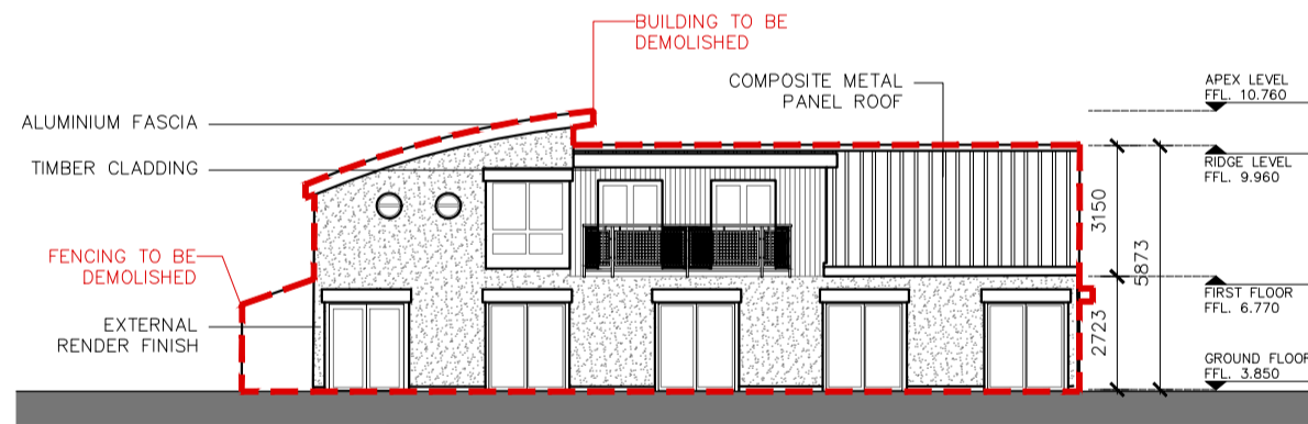
07 Poolbeg Yacht and Boat Club Existing North Elevation EX100 1:200
