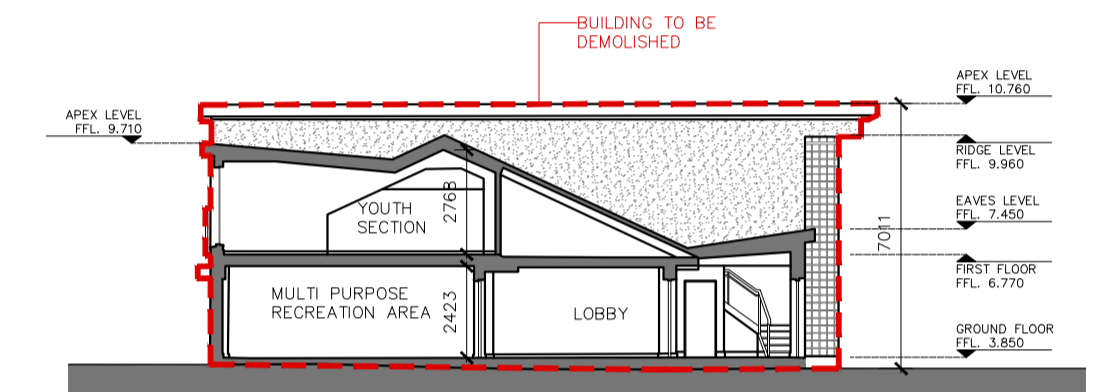
04 Poolbeg Yacht and Boat Club Existing Section AA EX100 1:200
