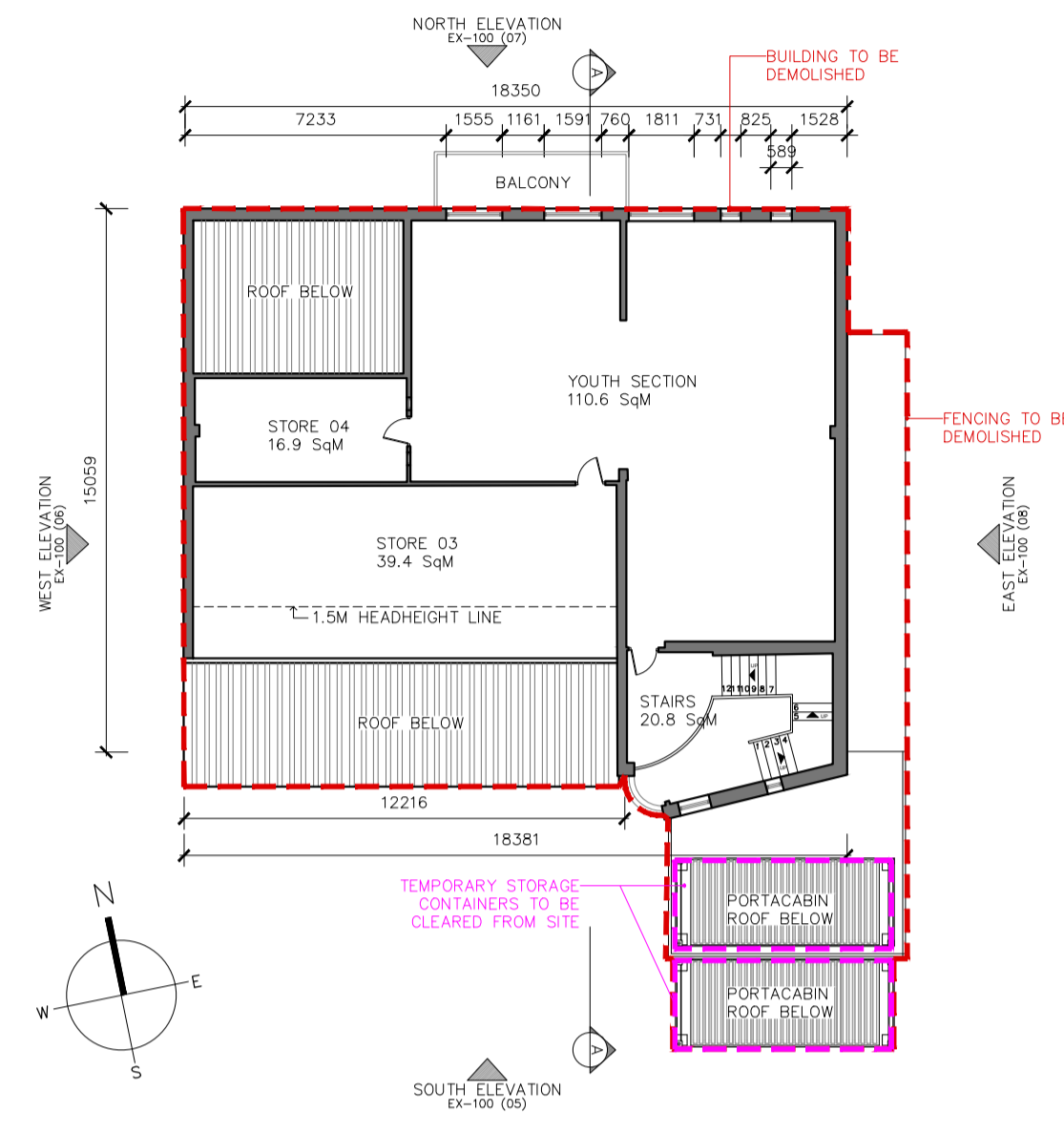
02 Poolbeg Yacht and Boat Club Existing First Floor Plan EX100 1:200
