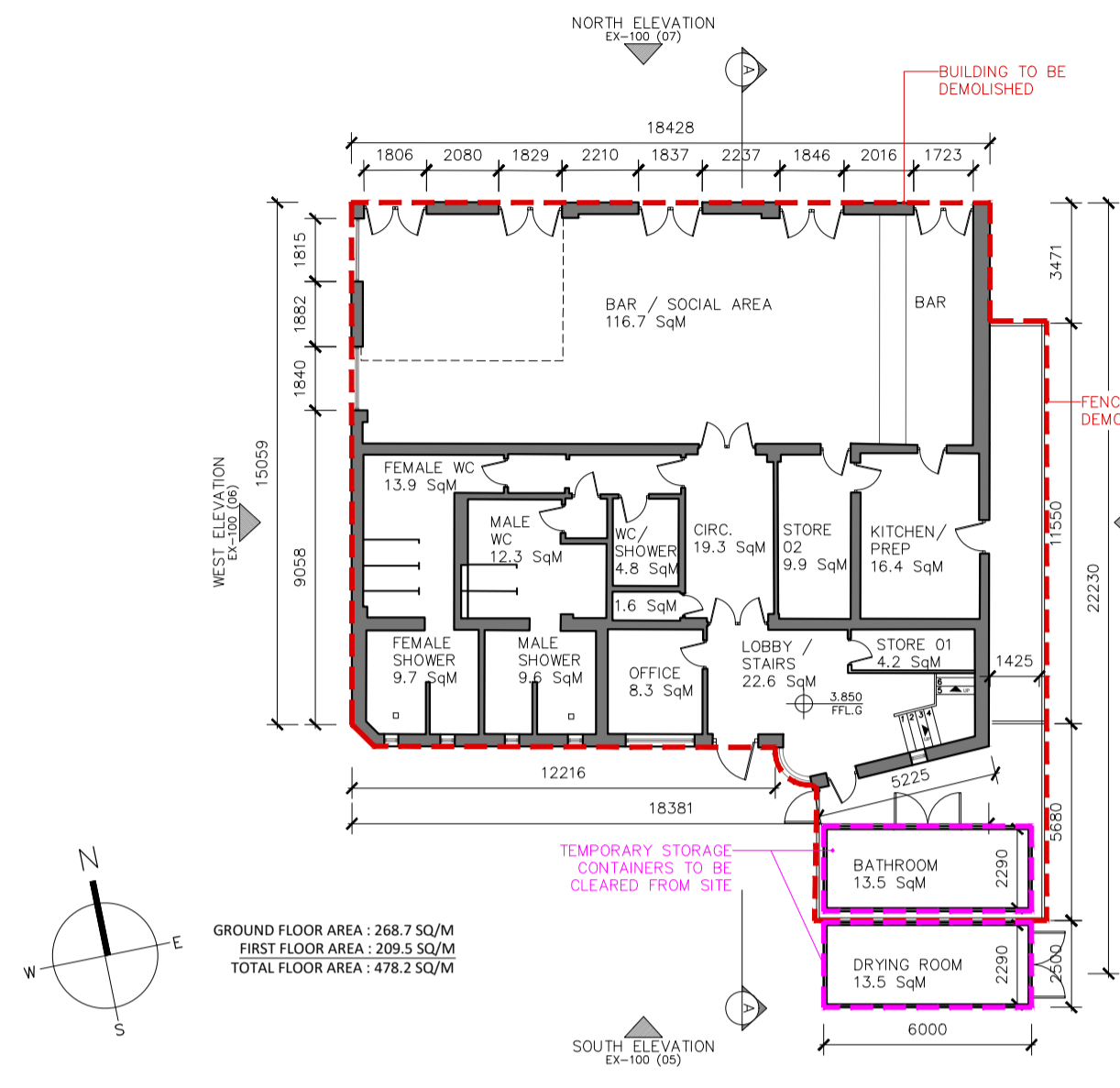
01 Poolbeg Yacht and Boat Club Existing Ground Floor Plan EX100 1:200
