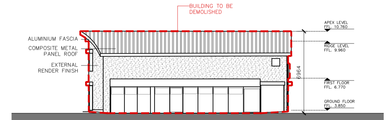
08 Poolbeg Yacht and Boat Club Existing East Elevation EX100 1:200
