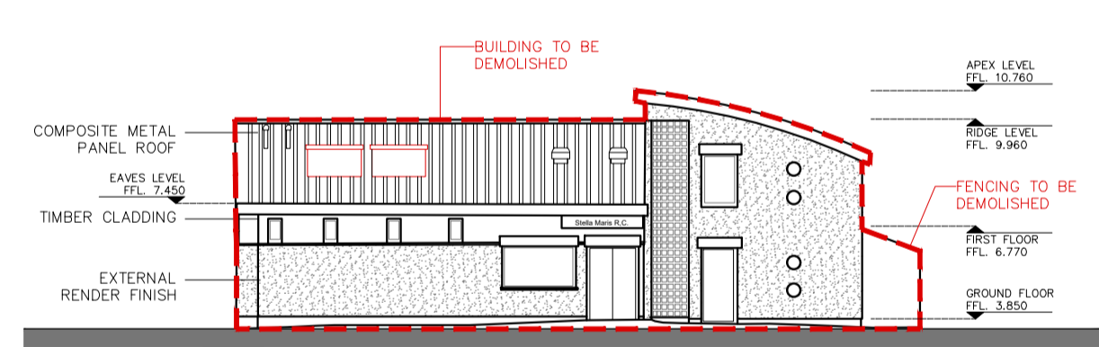
05 Poolbeg Yacht and Boat Club Existing South Elevation EX100 1:200
