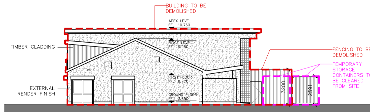
06 Poolbeg Yacht and Boat Club Existing West Elevation EX100 1:200
