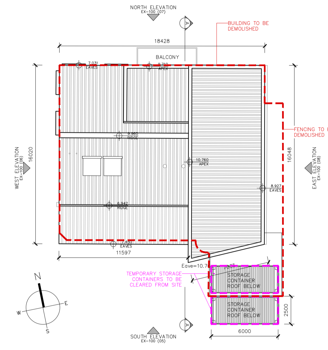
03 Poolbeg Yacht and Boat Club Existing First Floor Plan EX100 1:200
