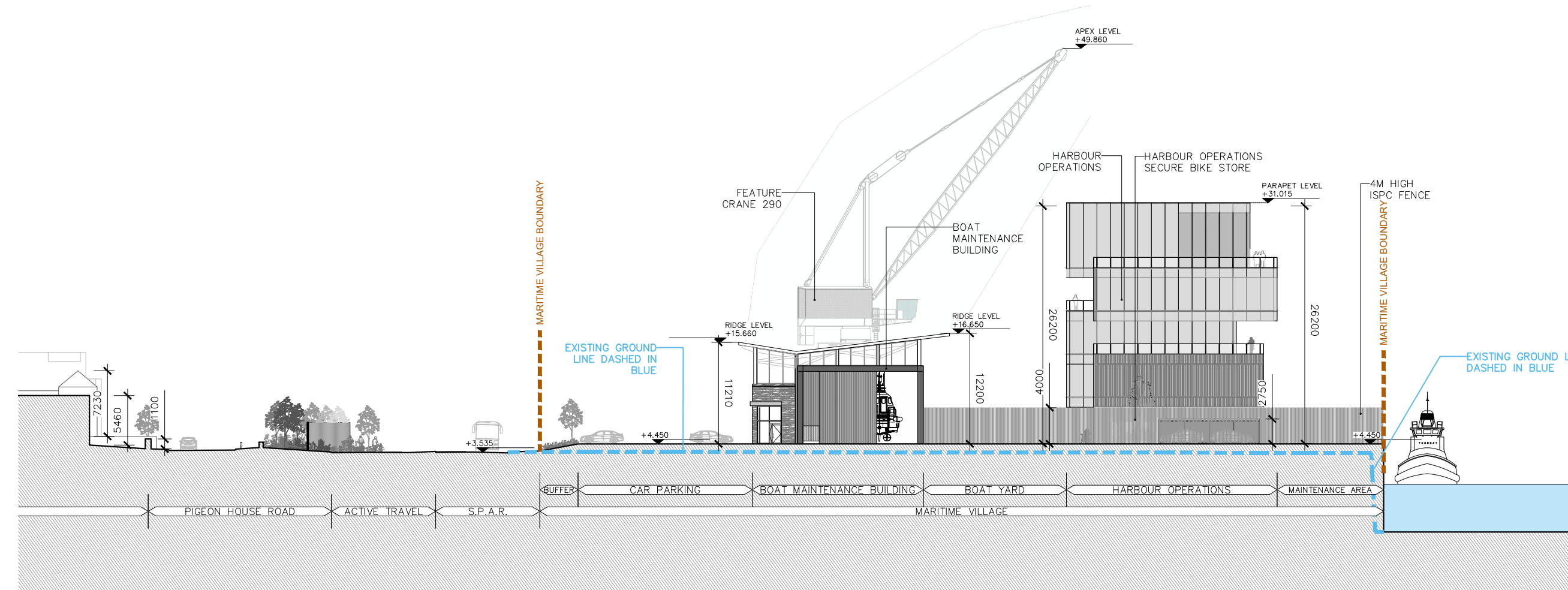
01 Proposed East Contiguous Elevation PA013 1:500
