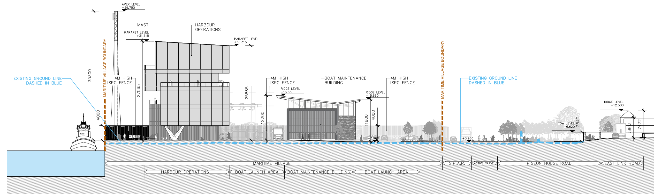
01 Proposed Site Section AA PA014 1:500
