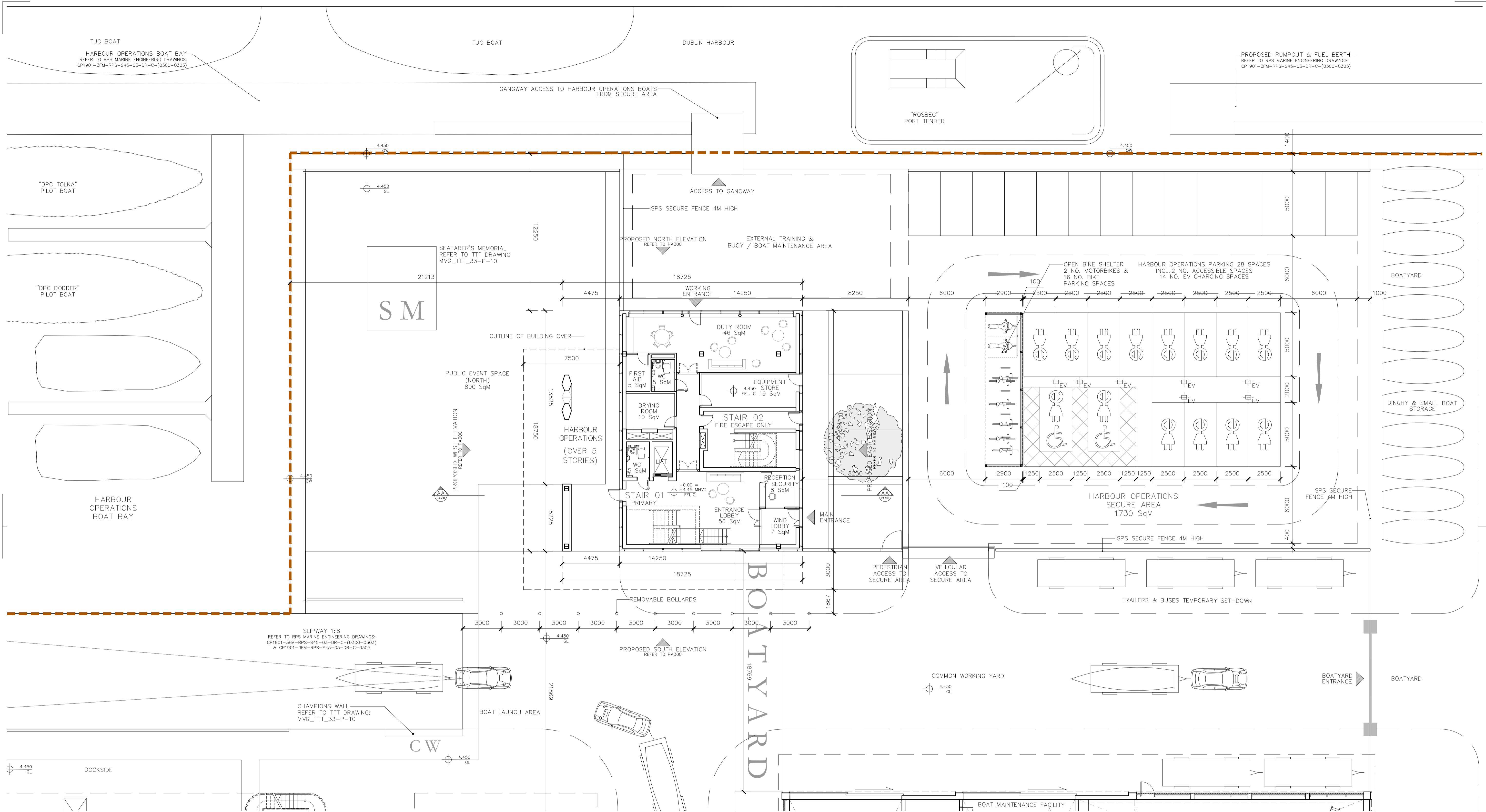
01 Proposed Harbour Operations Building - Site Plan PA100 1:200
