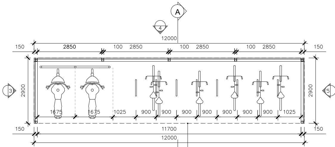
01 Proposed Bike Store 02 PA-402 1:100 Bike Store 02: Open bike shelter to accommodate 2 no. motorbike & 16 no. bike parking spaces *Note bike store is within Harbour Operations ISPS Secure Area
