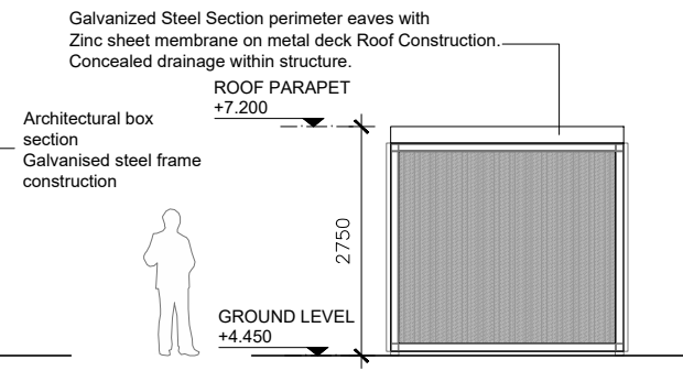
03 North Elevation PA-402 1:100
