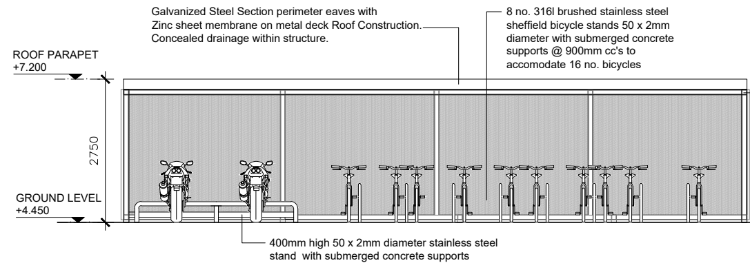
02 West Elevation PA-402 1:100
