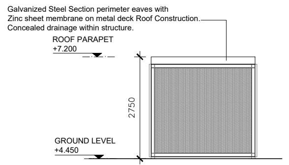
05 South Elevation PA-402 1:100
