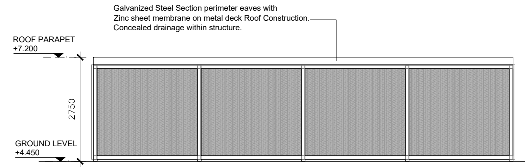
04 East Elevation PA-402 1:100
