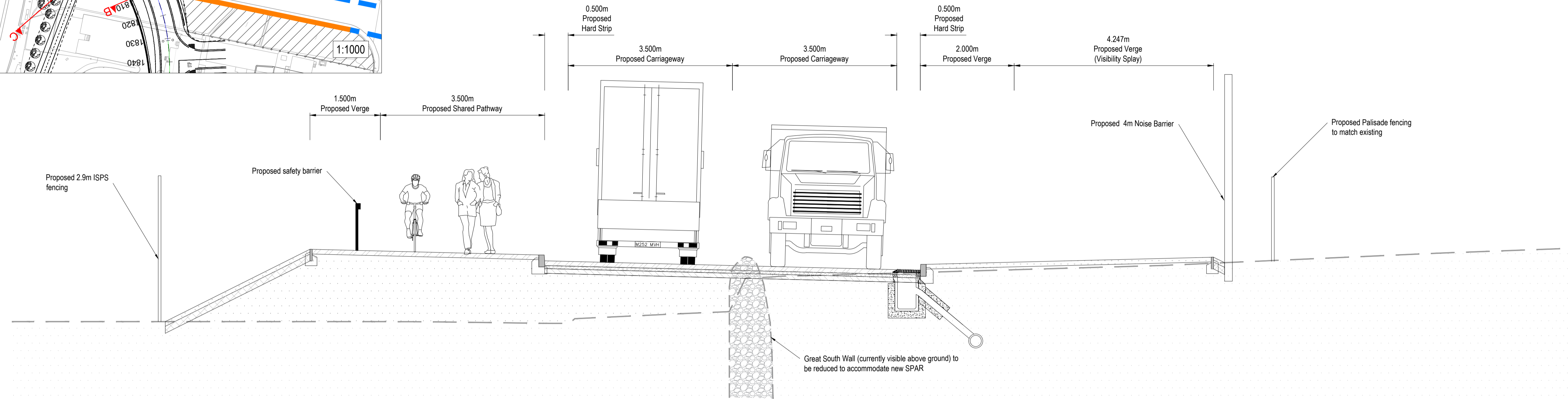
Typical Cross Section SPAR Section B-B 1:50
