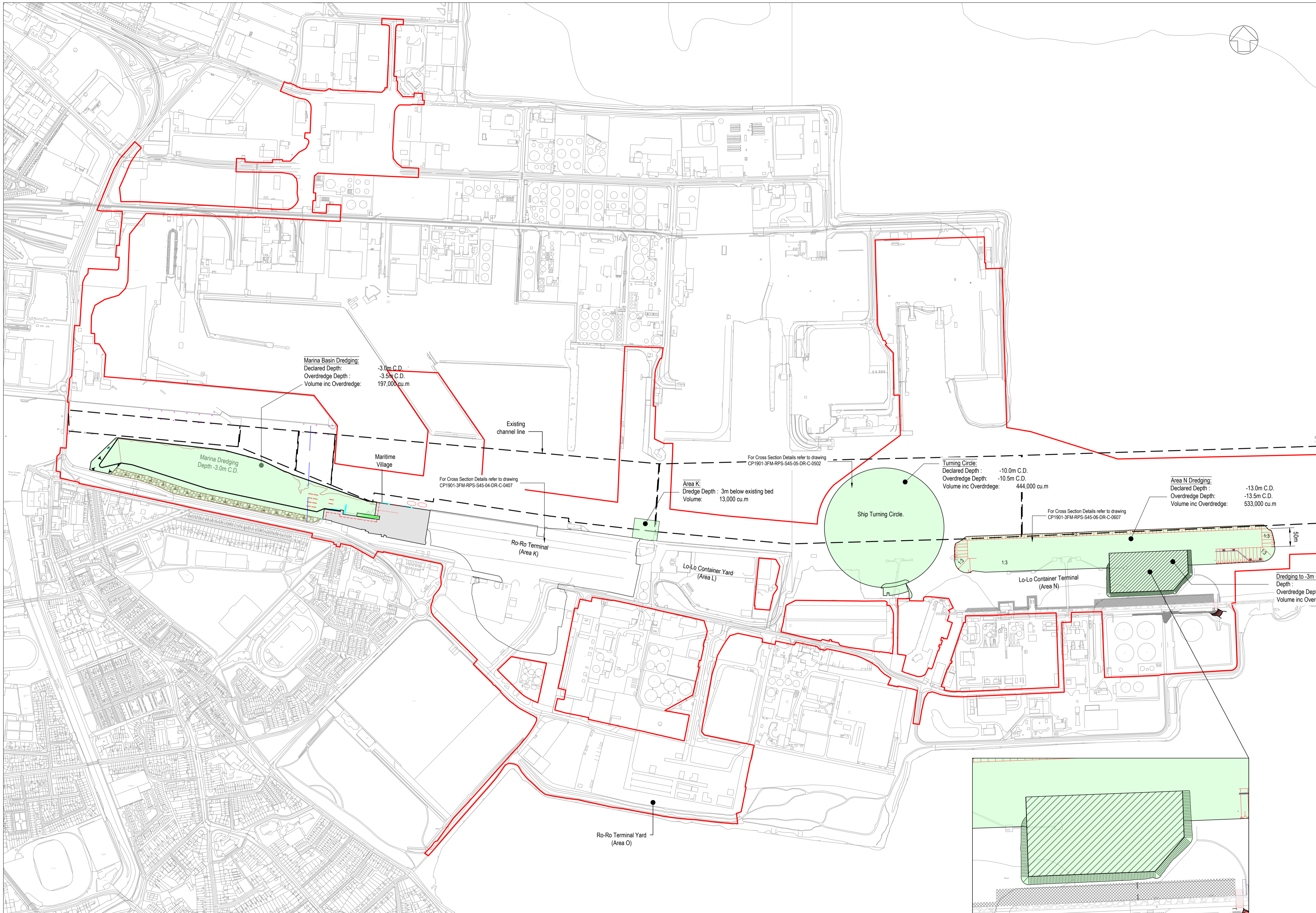
Dredge Layout (1:5000)
