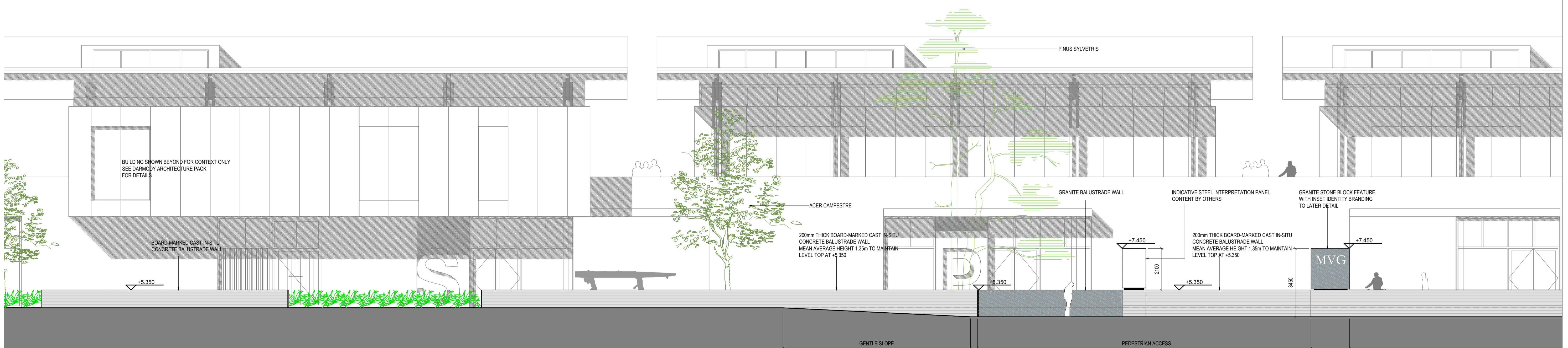
02. SECTION BB, SCALE 1:100
